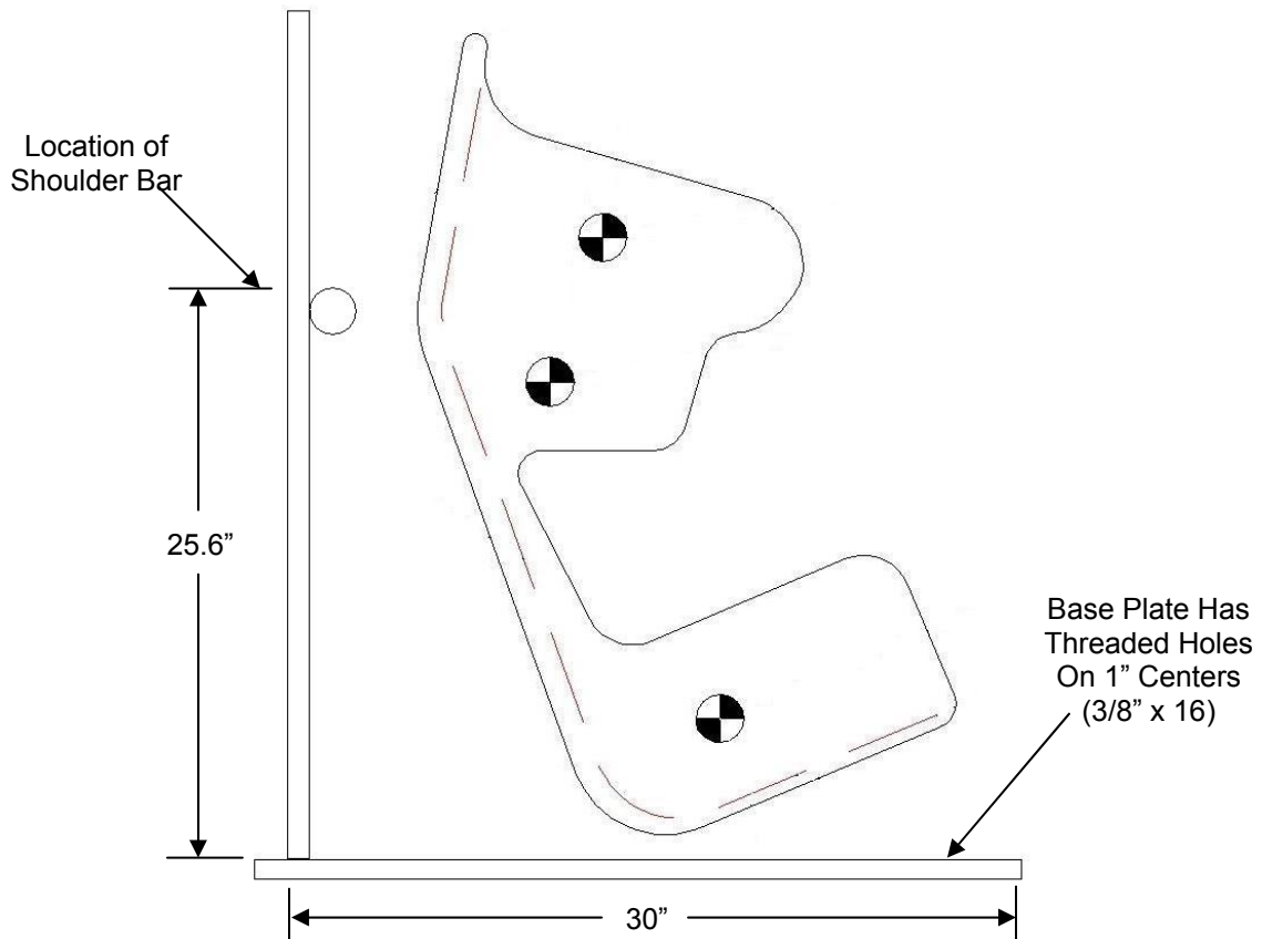
SFI Seat Test Fixture Envelope
