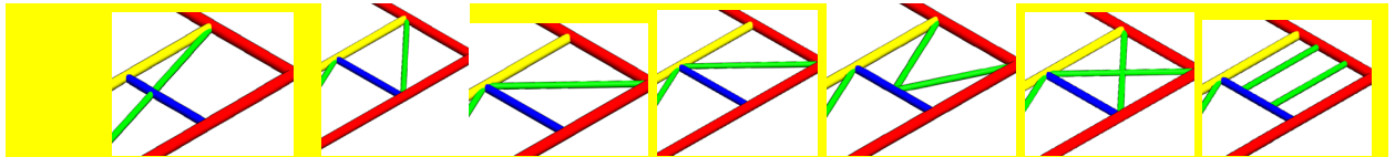
Outer Floor Triangulation Bar under-seat (#8A) options
